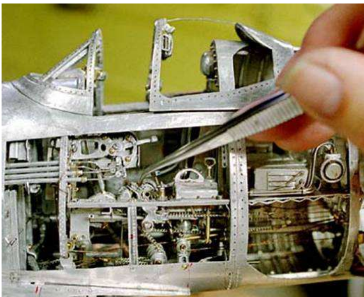
Using a tweezers, the controls can be moved. All cables and linkages are in place to work the wing control surfaces as well. Young Park has since carved a pilot's face and hands
